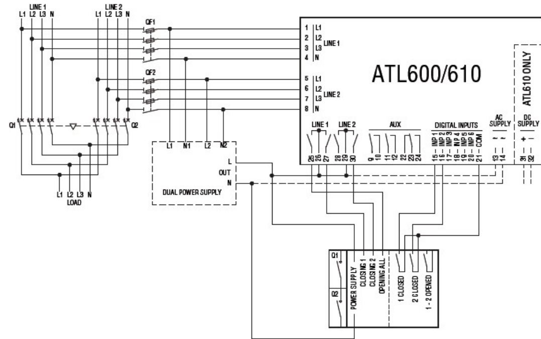
Connection diagrams Motorised changeover switches control
