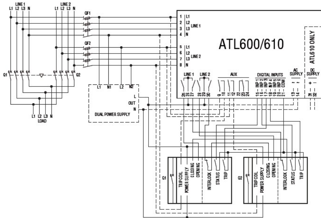
Connection diagrams Motorised breaker control
